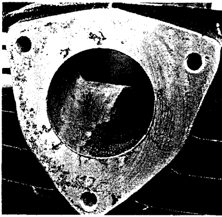
Sand-cast ports' interiors are rough, and will flow better when their walls are smoothed by filing.
