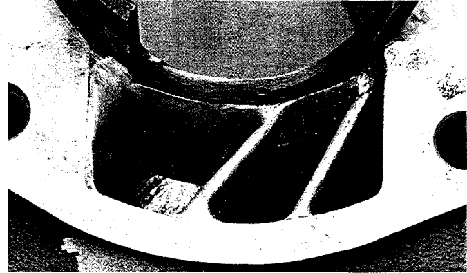
Work inside the transfer tunnels is most difficult, but also most effective.
