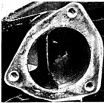
It's especially important that an exhaust port's walls be smooth, but don't thin the bridge.
