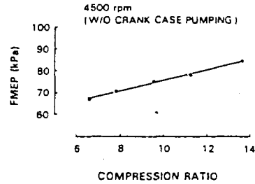
Fig. 7 Relationship between the Compression Ratio and the Mechanical Loss
