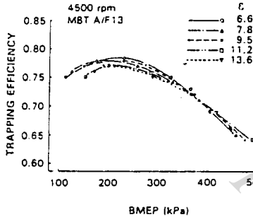
Fig. 4 Relationship between the Trapping Efficiency and BMEP
