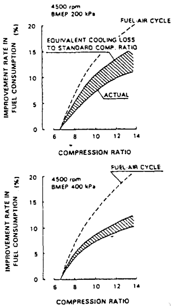
Fig. 9 Improvement Rate in Fuel Consumption without Increased Cooling Loss
