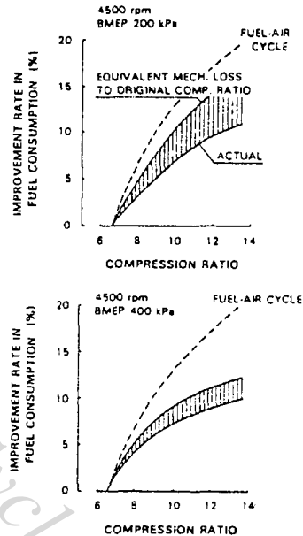
Fig. 8 Improvement Rate in Fuel Consumption without Increased Mechanical Loss
