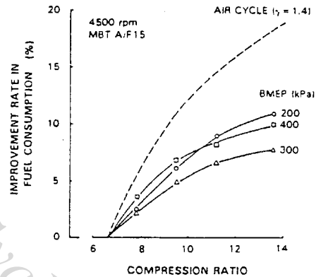
Fig. 2 Improvement Rate in Fuel Consumption at Various Loads
