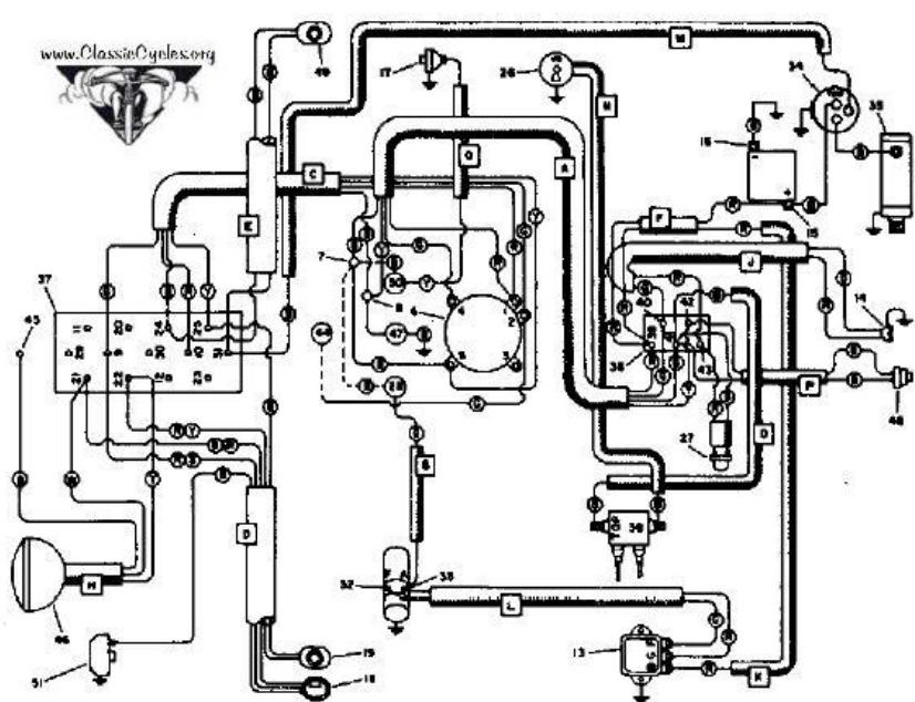
1965-67 Electra Glide
