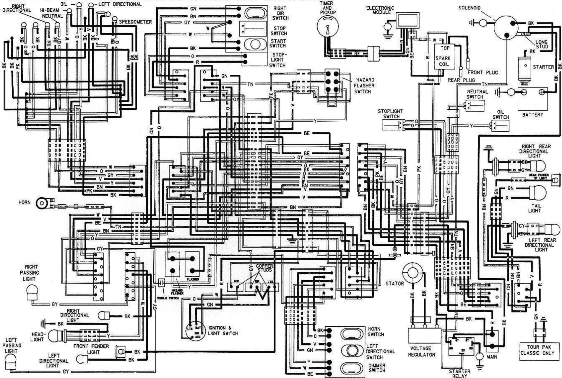
Typical wiring diagram for 1980 through 1983 FLT models (1983 FLHT shown) – later models similar
