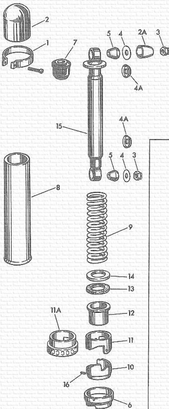
Figure 2F-37. 1966 & Earlier Rear Shock Absorber - Exploded View
